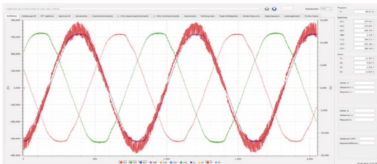
FIGURE 14: ELECTRIC VEHICLES NO. 1 AND NO. 2 ARE CONNECTED IN PARALLEL, STILL MEASURING AT VEHICLE NO. 1
