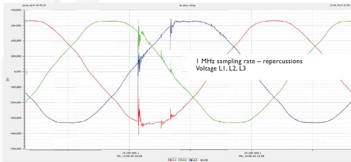
FIGURE 16: VOLTAGE TRANSIENTS AT ALL THREE PHASES
