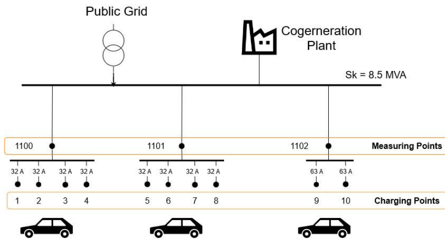
FIGURE 1: CIRCUIT DIAGRAM OF THE CHARGING STATION
