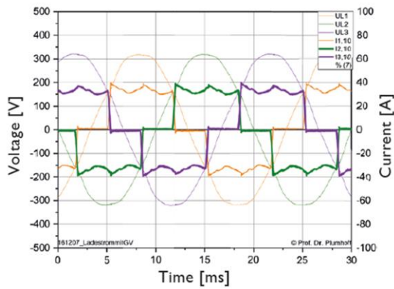
FIGURE 4: CHARGING WITH INDUCTIVE SMOOTHING
