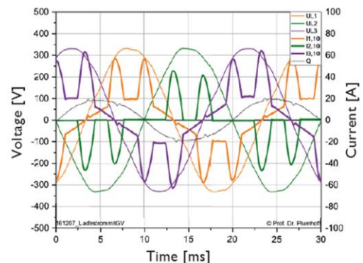
FIGURE 3: CHARGING WITH CAPACITIVE SMOOTHING
