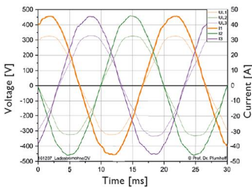
FIGURE 2: CHARGING CURRENT WITHOUT LIMIT VIOLATION
