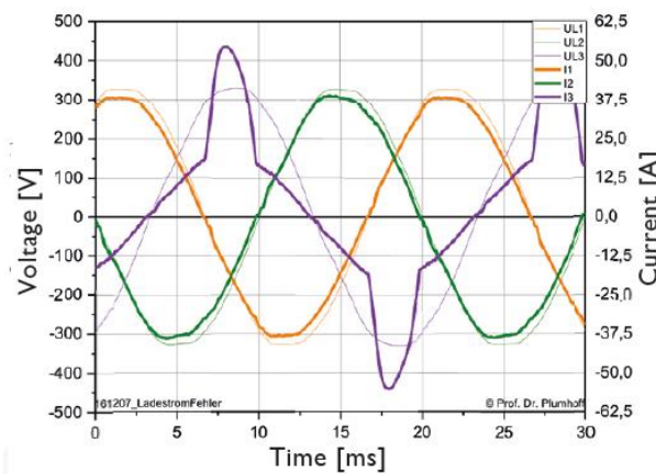
FIGURE 7: FAULTY CHARGING PROCESS
