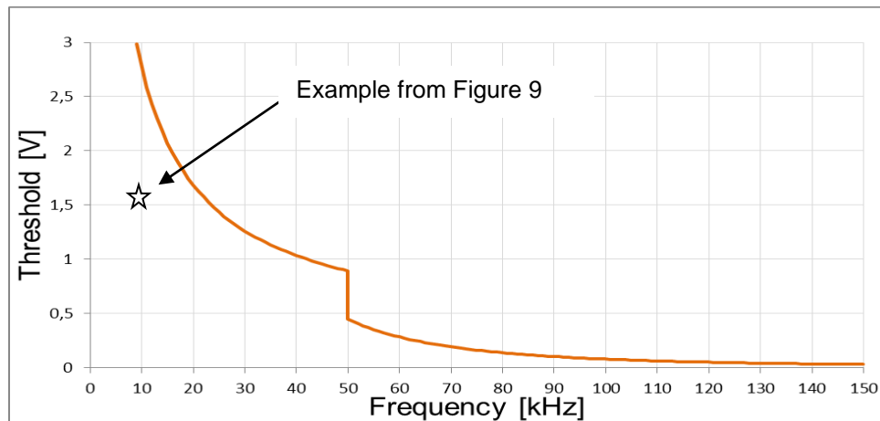
FIGURE 11: SUPRAHARMONIC THRESHOLDS OF IEC 61000-2-2 STANDARD
