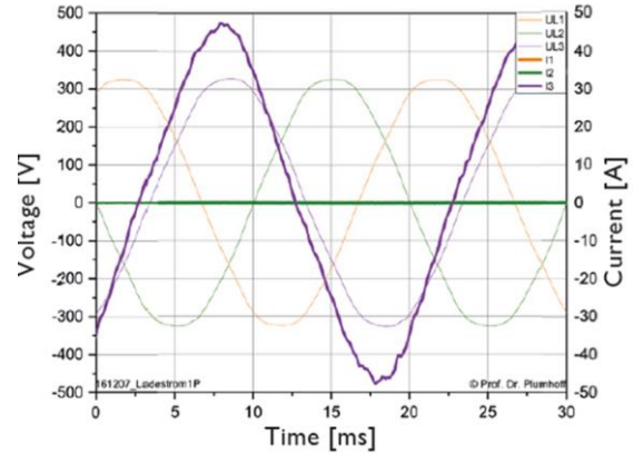
FIGURE 5: UNBALANCED CHARGING (7 kW, ONE PHASE)
